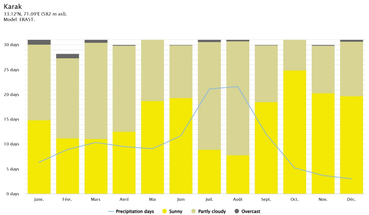
Figure 12: Cloudy, Sunny, and Precipitation Days Diagram showing concentration of rainfall during July–August.
