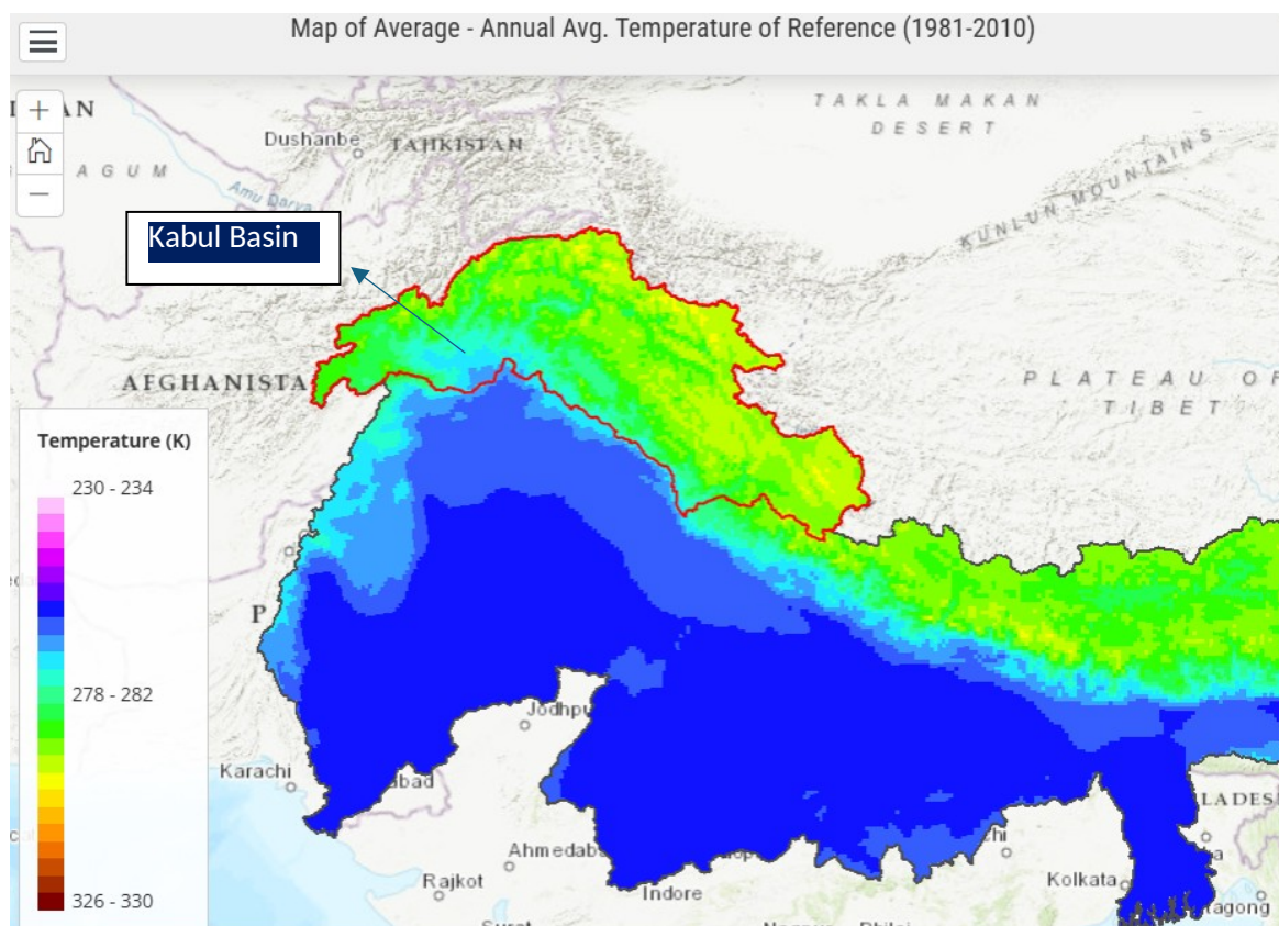
Figure 2: Map of average temperature of Upper Indus Basin (1981-2010) 30
