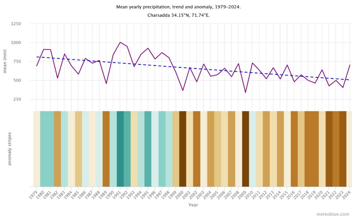
Figure 11: Yearly Precipitation Change in Charsadda (1979–2024) showing high variability with a slight drying trend.
