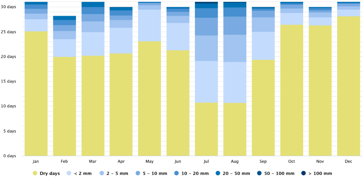
Figure 14: Precipitation Amounts Diagram illustrating clustering of heavy rainfall days in the monsoon season.
