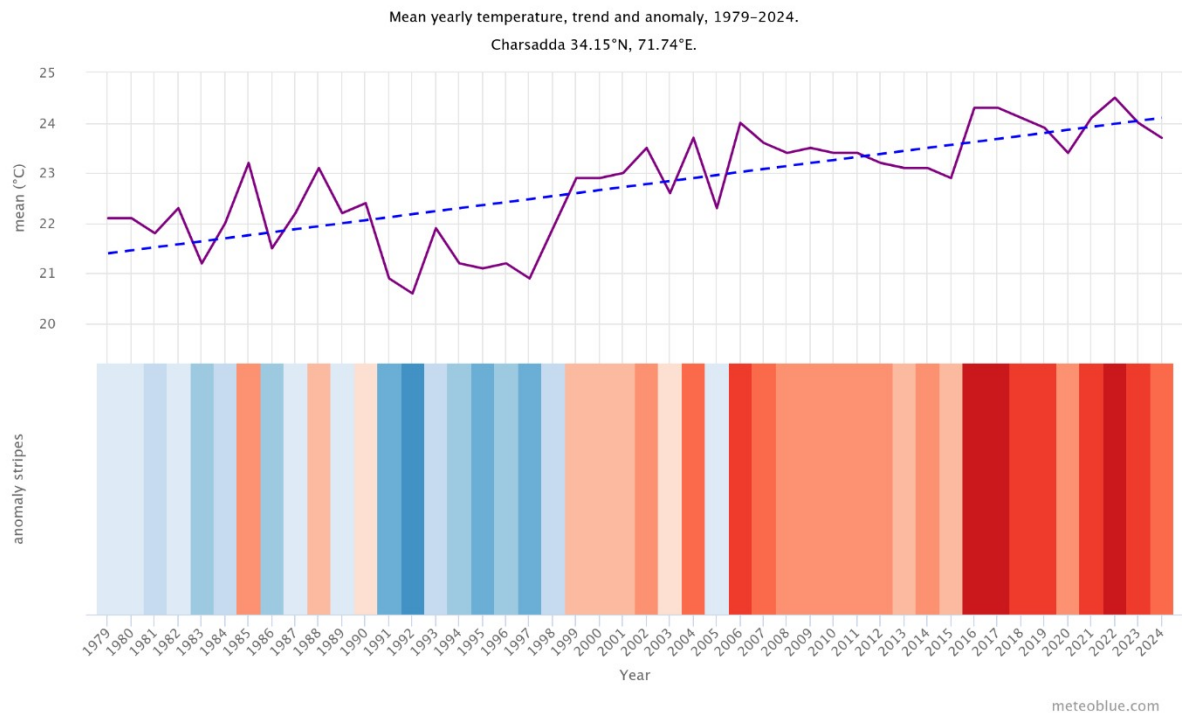
Figure 7: Yearly Temperature Change in Charsadda (1979–2024) showing consistent warming with predominance of hotter years since 2000.
