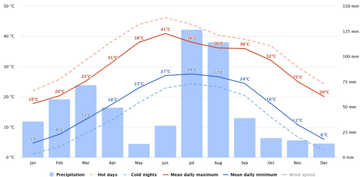
Figure 12: Climate Diagram of Average Temperatures and Precipitation highlighting extreme summer heat and monsoon rainfall peaks.
