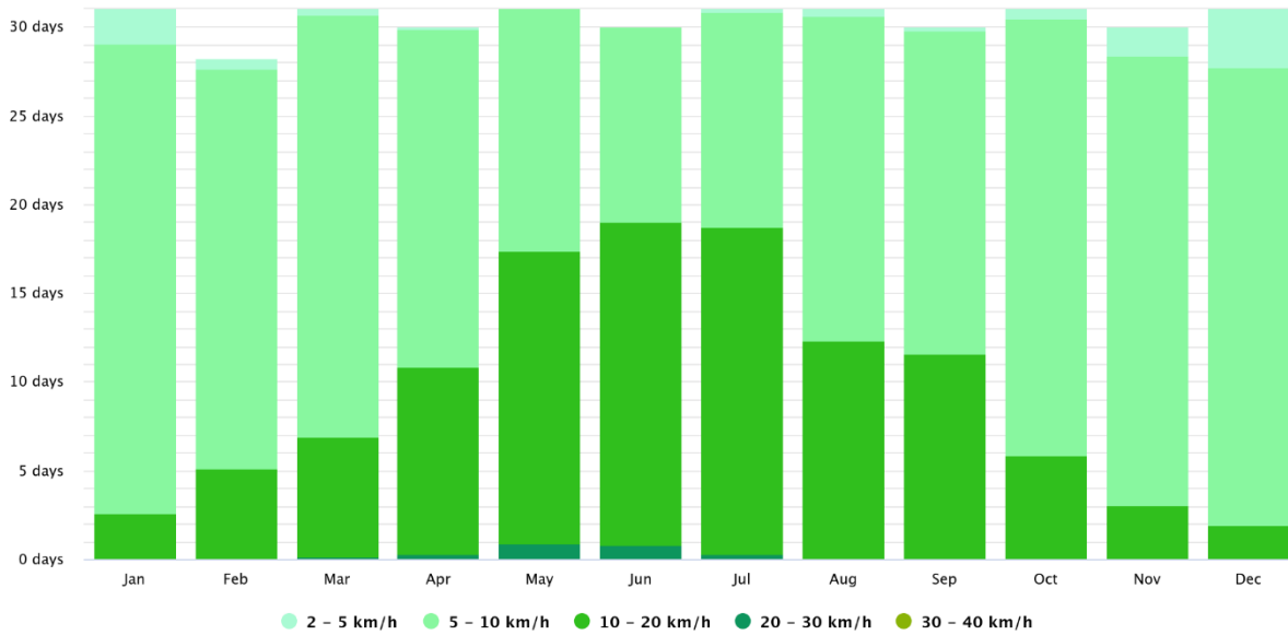
Figure 15: Wind Speed Diagram showing moderate but seasonally variable wind conditions.
