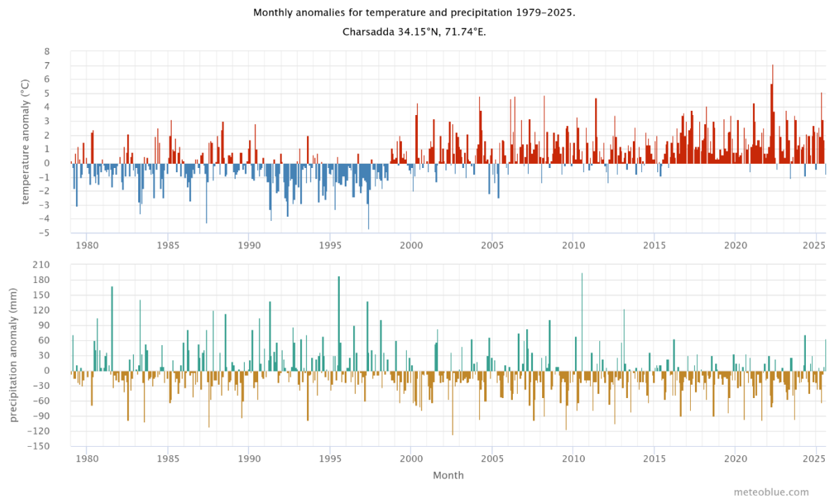
Figure 8: Monthly Temperature and Precipitation Anomalies (1979–2024) illustrating a clear shift toward warmer-than-normal months in recent decades.
