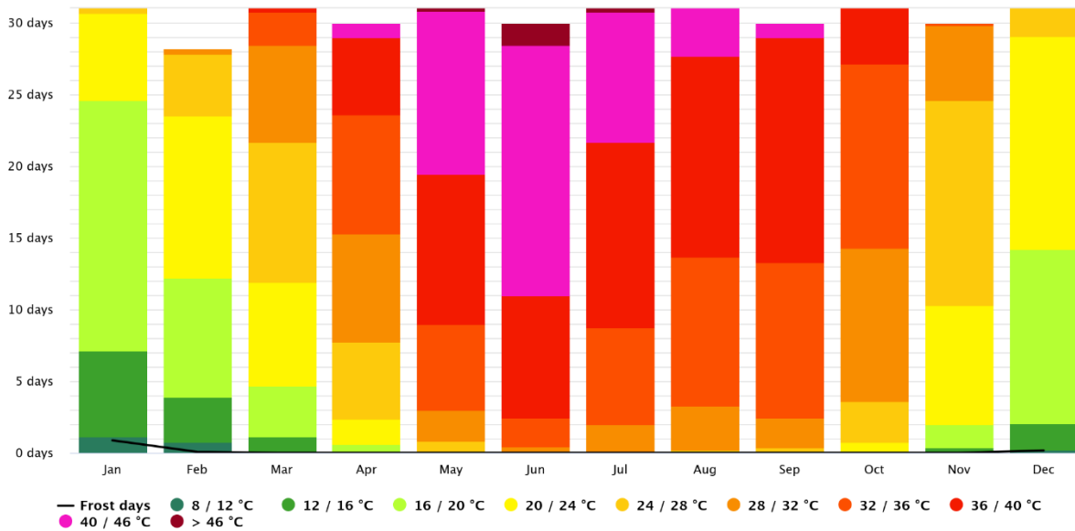
Figure 9: Maximum Temperature Diagram highlighting the high frequency of extreme heat days during May-June.
