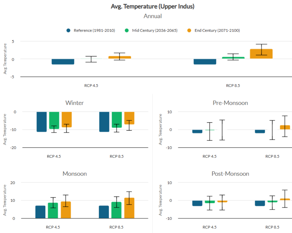
Figure 3: Projected changes in average temperature over the Upper Indus Basin under different Representative Concentration Pathways (RCPs) and time horizons.
