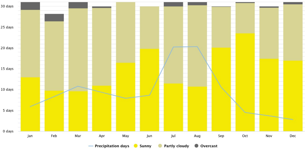
Figure 13: Cloudy, Sunny, and Precipitation Days Diagram showing high concentration of rainy days during July–August.
