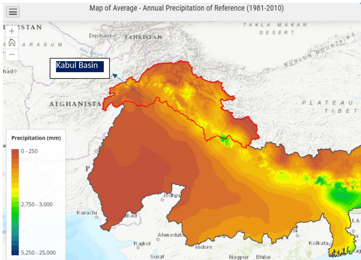
Figure 4: Map of average precipitation of Upper Indus Basin (1981-2010)
